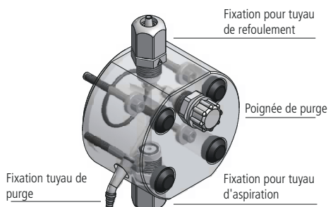
fig.7b. PMMA pump head connections.
