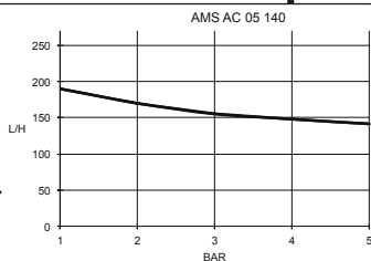
T pump head
