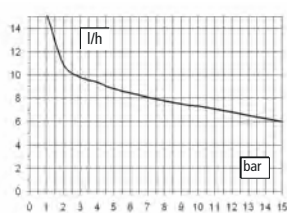
Pump head MA
