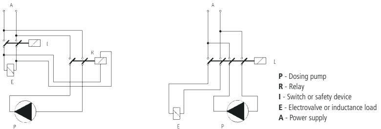
Fig. 9. Electrical installation.
