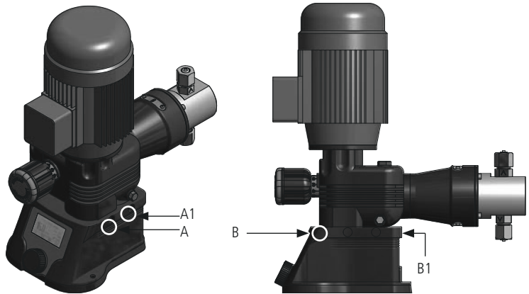
Fig. 5. Default to alternative position: move screws from A to A1 and from B to B1.
