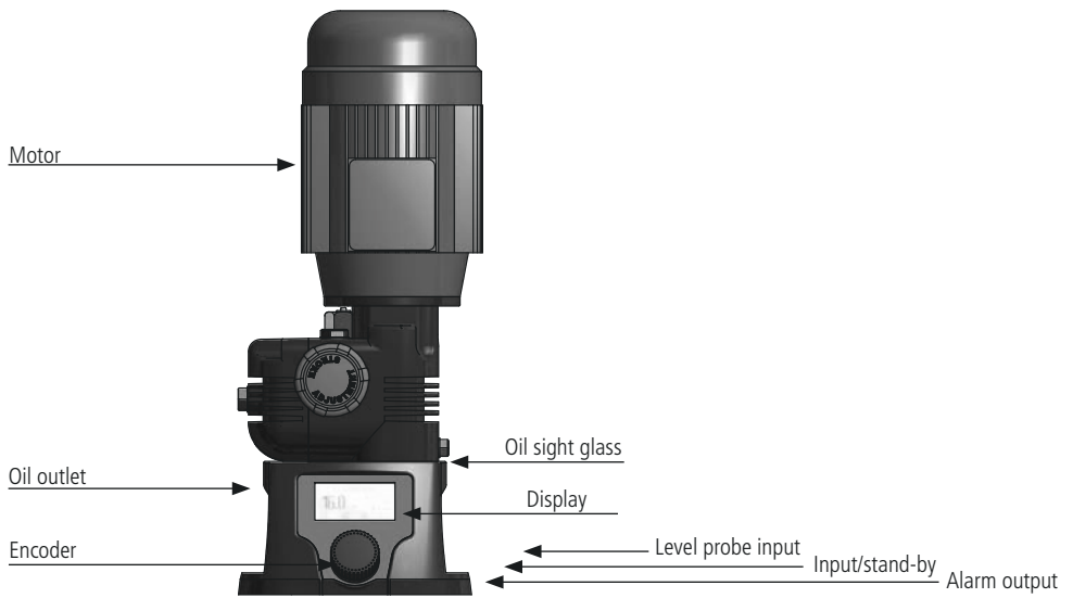
Fig. 2. PRIUS P MF pump
