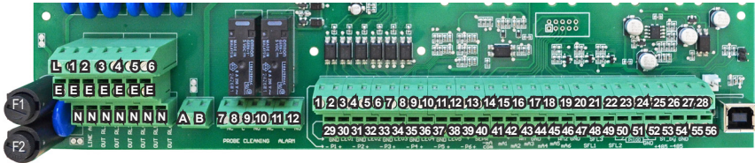
Electrical Connections
