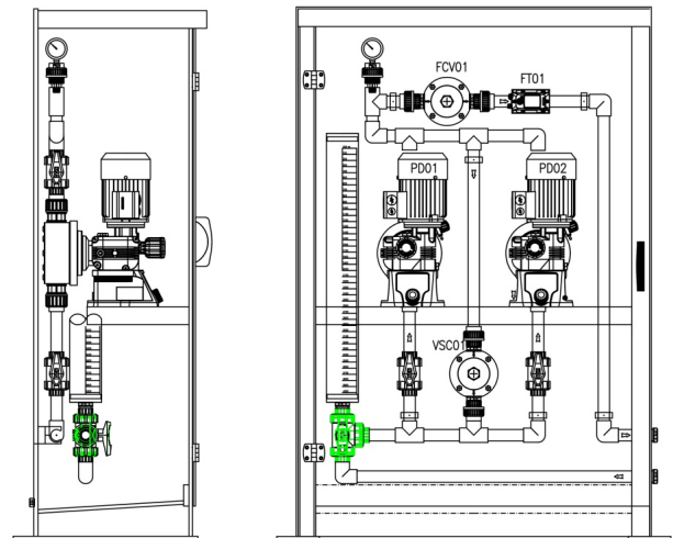
Fig. 3 - Skid Safety Box
