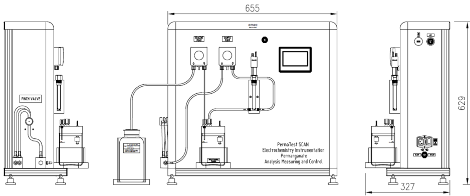
Fig. 1 - Instrumentation panel
