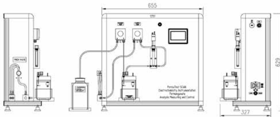
Fig. 1 - Instrumentation panel
