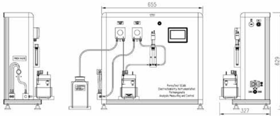
Fig. 1 - Instrumentation panel
