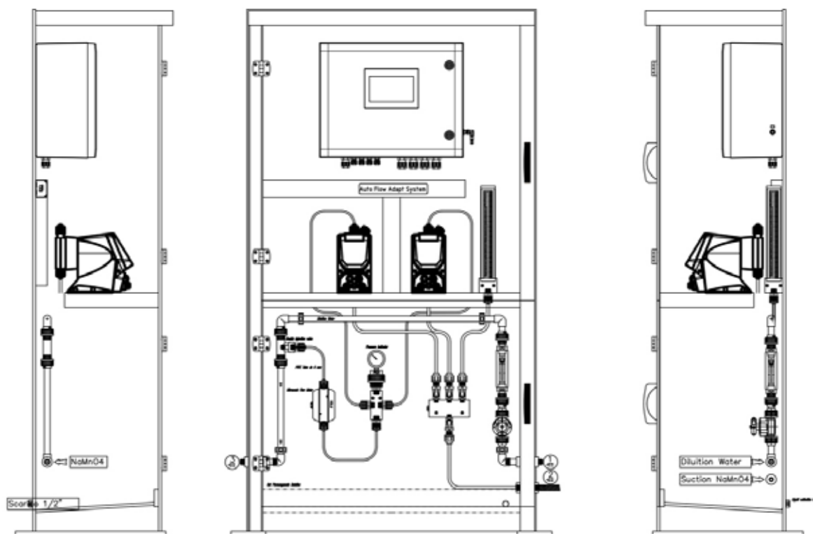
Fig. 1 - Instrumentation panel
