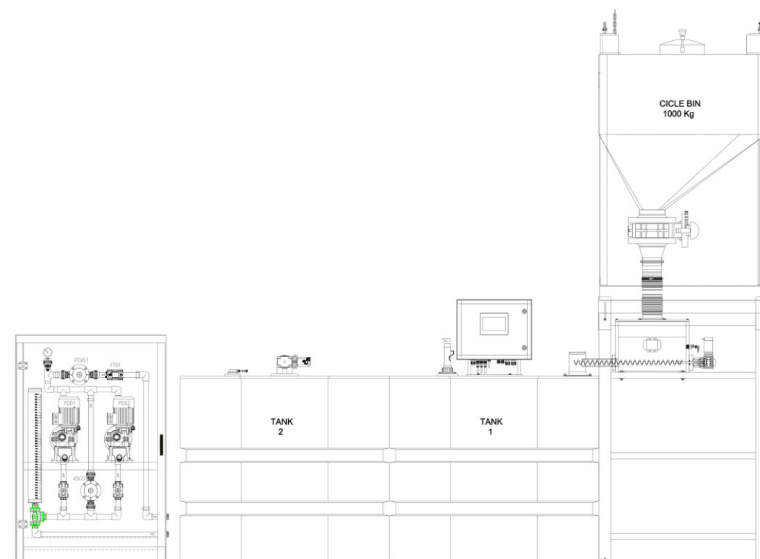
Fig. 1 - Schema PermaDos CB + Skid Safety Box
